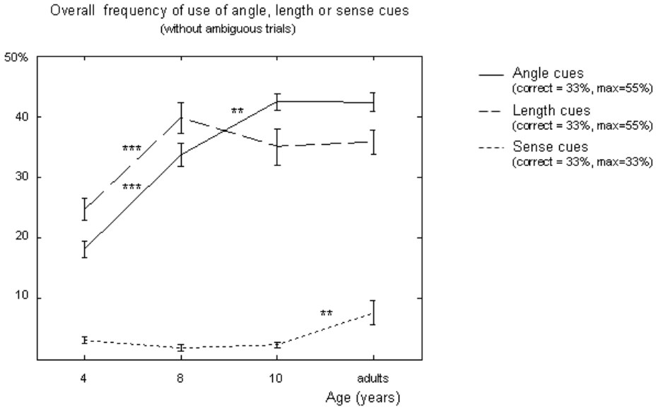
Figure 9. Overall frequency of use of angle, length and sense cues. A compound measure was created, to estimate how often trials are responded using angle (resp. length, sense) cues, either being an angle (resp. length, sense) trial responded correctly, or because a smallest/largest/right angle (resp. length) was chosen in an interference trial. Ambiguous trials, which could have been attributed to either or the other of these cues, were removed from this analysis. The frequencies evolved differently with age, thus creating a significant interaction. The stars refer to differences between age groups for each type of cue (**: p < 0.01 ; ***: p < 0.001 ).
